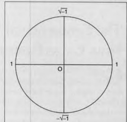
FIGURE IV. The unit of action in Gauss's complex domain.
