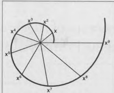
FIGURE III. A succession of algebraic powers is generated by a self-similar spiral.
