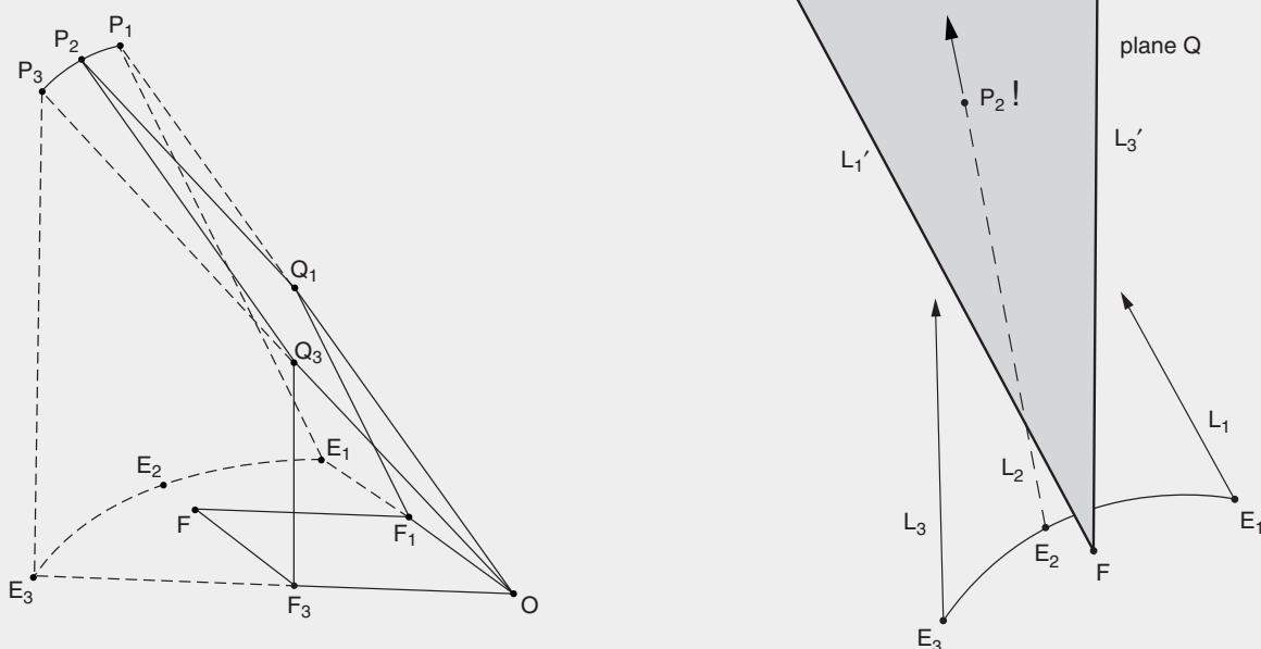
FIGURE 14.3. In Chapter 11, we located Ceres' position P_2 on plane Q , using a construction pivoted on the discrepancy between the curvatures of the orbits of Earth ( E_1E_2E_3 ) and Ceres ( P_1P_2P_3 ).
