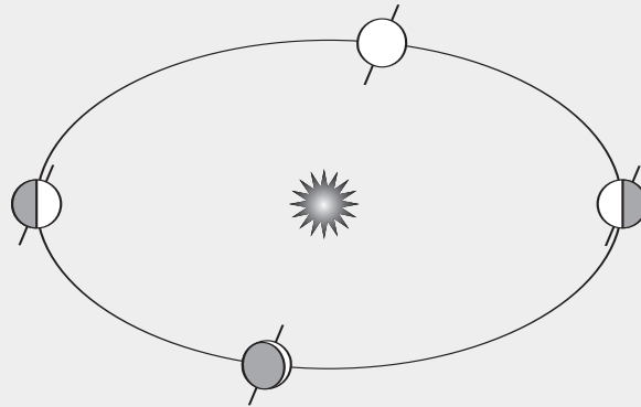
FIGURE 2.4. Orbit of Earth (yearly).
