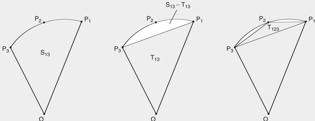
FIGURE 14.12. S_{13} is (to a first order of approximation) very nearly equal to T_{13} + T_{123} .
