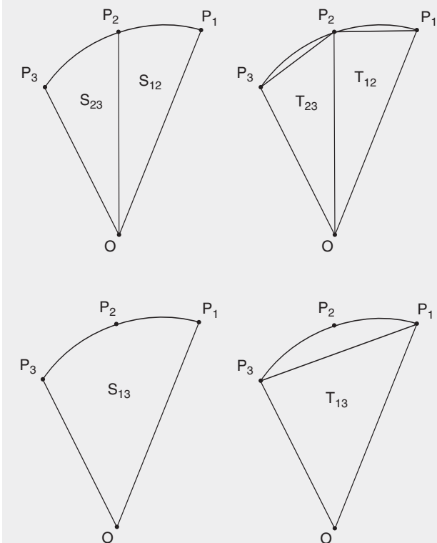
FIGURE 10.4. Orbital sectors S_{12}, S_{23}, S_{13} , and their corresponding triangular areas T_{12}, T_{23}, T_{13} .
