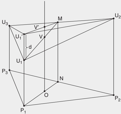
FIGURE 13.6. Tilt the plane of the U 's up from U_1 to U_1' , to generate V' . What is the functional relationship between
