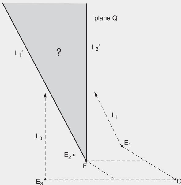
FIGURE 11.5. P_2 must lie on plane Q constructed at point F . But where?
