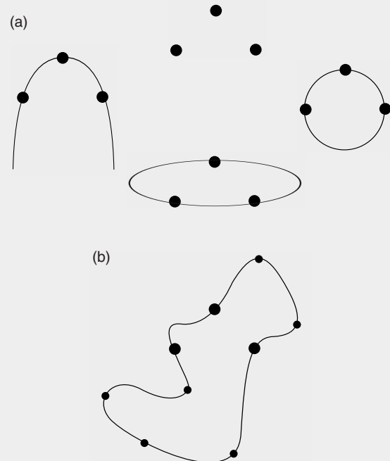
FIGURE 1.5. (a) Here are just a few of the curves that can be drawn through the same three points. (b) With more observation points, we may find that the curve is not as anticipated.
