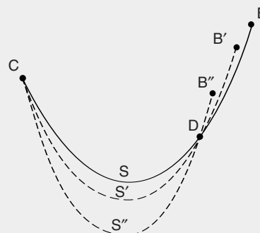
FIGURE 4.5. Only one unique position of B produces the exact tension and curvature of catenary CD . Different parts of a given catenary are local expressions of the whole, sharing a common internal characteristic.
