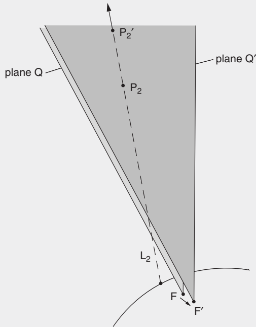
FIGURE 12.5. Owing to the extremely flat angle which the line L_2 makes to the plane Q , a slight shift in the position of F (from F to F' ) causes a much larger change in the point of intersection with L_2 (from P_2 to P_2' ).
