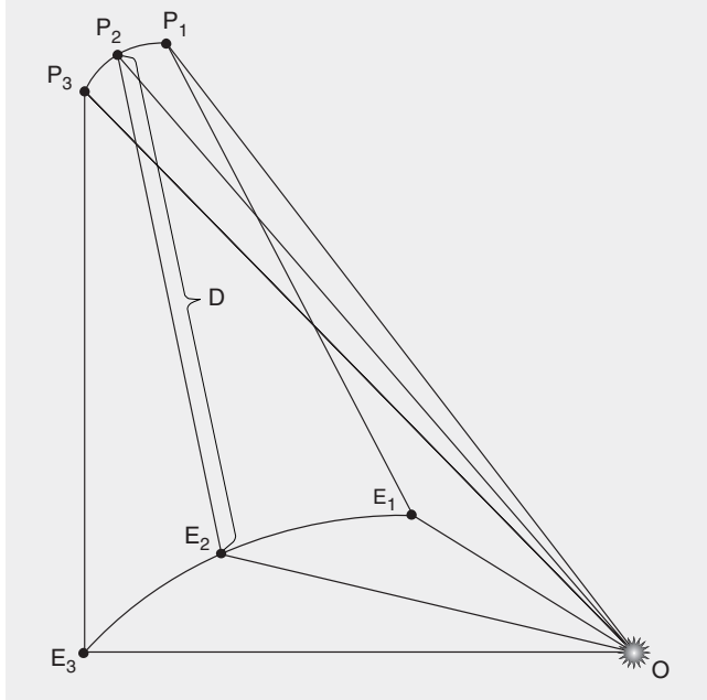
FIGURE 9.3. Gauss's immediate goal: determine distance D from E_2 to P_2 .
