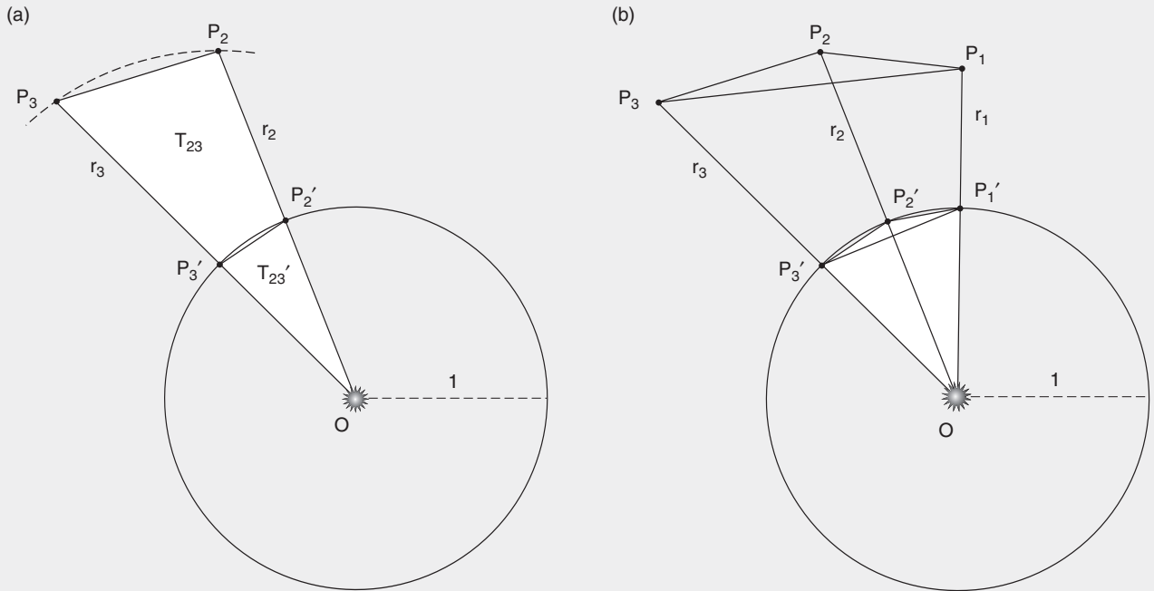
FIGURE 14.9. “Reduction” of relationships on non-circular orbit to relationships in a circle. (a) The area of triangle T_{23}' , obtained by projecting P_2 and P_3 onto the circle of unit radius, is equal to T_{23}'(r_2 \times r_3) . (b) Similarly for triangles T_{12}' and T_{13}' . The original apex angles at the sun are preserved, but the lengths are all reduced to 1.
