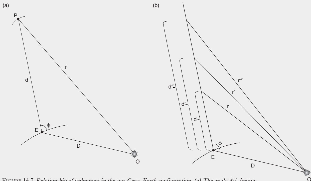
FIGURE 14.7. Relationship of unknowns in the sun-Ceres-Earth configuration. (a) The angle \phi is known from Piazzzi’s observations, and the Earth-sun distance D is also known. This defines a functional relationship between the unknown Earth-Ceres distance d and the unknown sun-Ceres distance r , as shown in (b). (b) To each hypothetical value of r , there corresponds a unique value of d , consistent with the known values of \phi and D .
