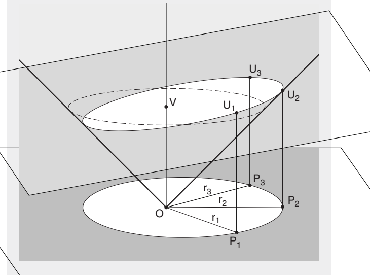
FIGURE 16.1. The elliptical orbit is easily determined from P_1, P_2, P_3 , by drawing the plane through the corresponding points U_1, U_2, U_3 (whose heights are the distances r_1, r_2, r_3 now known). However, Gauss rejected that direct method as being too prone to error when P_1, P_2, P_3 are close together.
