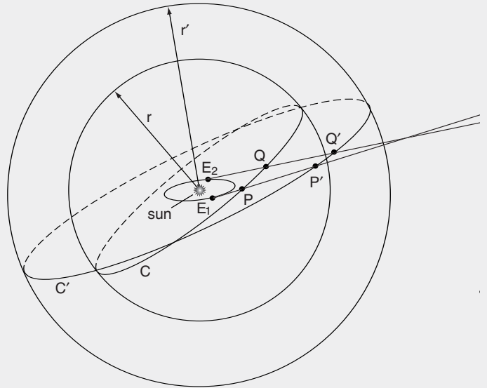
FIGURE 3.2. Method to determine the orbit of Ceres, on the assumption that the orbit is circular. Two sightings of Ceres define two lines of sight coming from the Earth positions E_1 , E_2 (the Earth's positions at the moments of observation). A sphere around the sun, of radius r , intersects the lines of sight in two points P, Q , which lie on a unique great circle C on that sphere. A sphere of some different radius r' would define a different set of points P', Q' and a different hypothetical orbit C' . Determine the unique value of r , for which the size of the arc PQ agrees with the rate of motion a planet would really have, if it were moving according to Kepler's laws on the circular orbit C over the time interval between the given observations.
