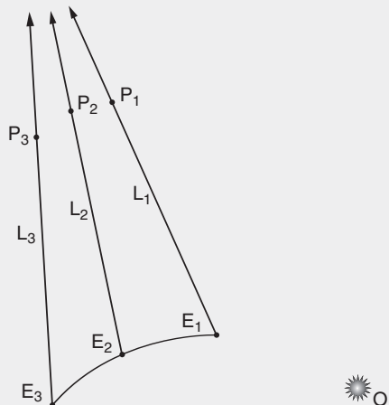
FIGURE 9.1. Positions of the sun ( O ), Earth ( E ), and Ceres ( P ), at the three times of observation. P_1, P_2, P_3 must lie on lines of sight L_1, L_2, L_3 , but their distances from Earth are not known.
