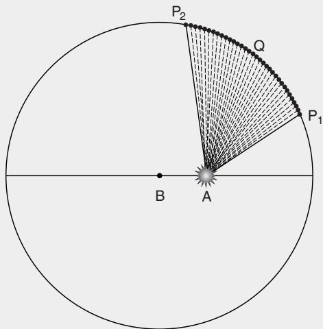
FIGURE 5.3. Assuming the “momentary” orbital velocities are inversely proportional to the radial distances, Kepler tries to “add up” the radii to determine how much time the planet needs to go from one point of the orbit to another.
