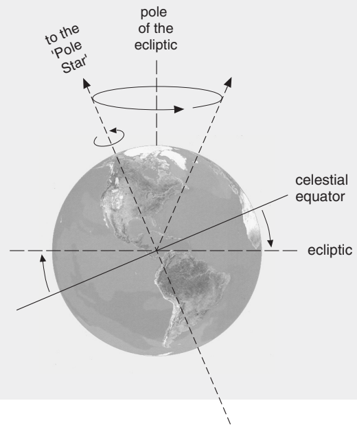
FIGURE 2.6. Precession of the equinoxes (period 25,700 years). The "precession" appears as a gradual shift in the apparent positions of rising and setting stars on the horizon, as well as a shift in position of the celestial pole. This phenomenon arises because Earth's axis of rotation is not fixed in direction relative to its orbit and the stars, but rotates (precesses) very slowly around an imaginary axis called the "pole of the ecliptic," the direction perpendicular to the ecliptic plane (the plane of the Earth's orbit).
