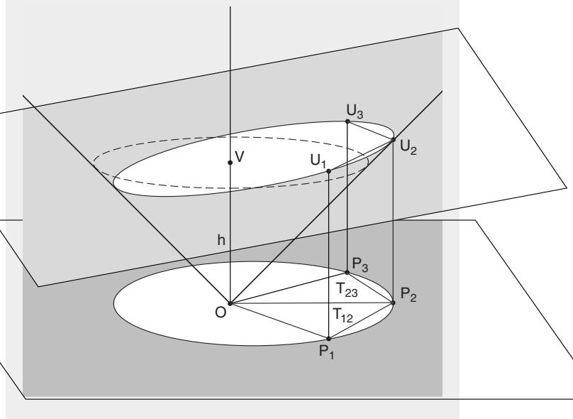
FIGURE 12.8. What is the relationship between the triangular areas T_{12}, T_{23}, T_{13} and height h of the point V ?
