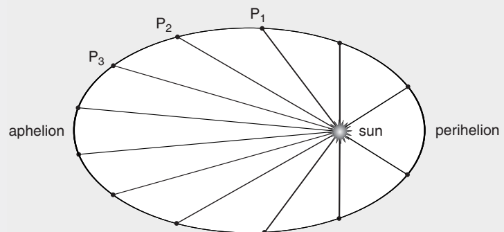
FIGURE 7.2. Kepler's constraint for motion on an elliptical orbit. The ratios of elapsed times are proportional to the ratios of swept-out areas. In equal time intervals, therefore, the areas of the curvilinear sectors swept out by the planet, will be equal—even though the curvilinear distances traversed on the orbit are constantly changing. In the region about perihelion, nearest the sun, the planet moves fastest, covering the greatest orbital distance; whereas, at aphelion, farthest from the sun, it moves most slowly, covering the least distance. This constraint is known as Kepler's "area law," later referred to as his "Second Law."
