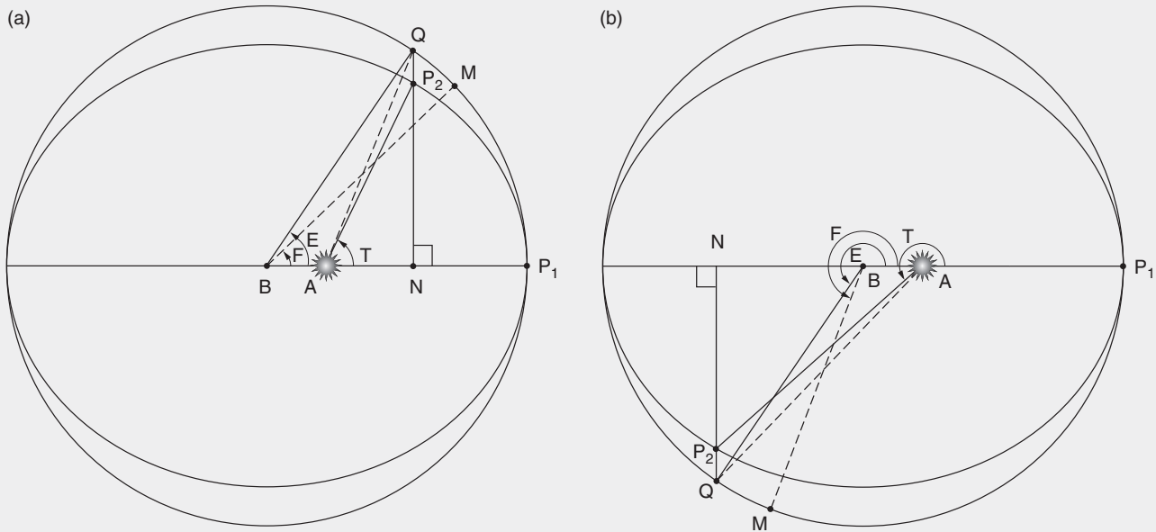
FIGURE 6.4. Non-uniform motion in an elliptical orbit is characterized by the “polyphonic” relationship between the “eccentric anomaly” (angle E ), “true anomaly” (angle T ), and “mean anomaly” (angle F ). (a) As the planet moves from perihelion to aphelion, the true anomaly is greater than the eccentric, which is greater than the mean. (b) After the planet passes aphelion, these relationships are reversed.
