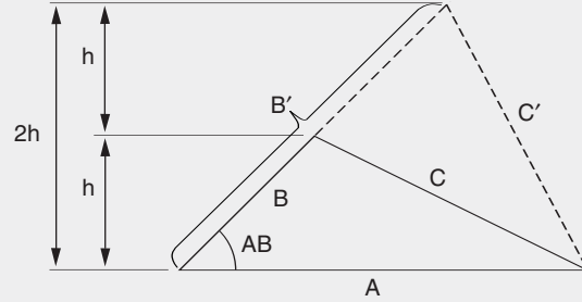
FIGURE 14.8. Doubling a side of a triangle, while keeping the adjacent side and angle constant, doubles the area of the triangle.
