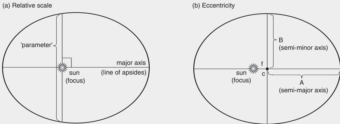
FIGURE 2.2. (a) The relative scale of the orbit can be measured by the line perpendicular to the line of apsides, drawn through the focus (sun). This line is known as the “parameter” of the orbit. (b) The eccentricity is measured as the ratio of the distance f from the focus to the center of the orbit (point c , the midpoint of the major axis) divided by the semi-major axis A . For the circle, in which case the focus and center coincide, f = 0 ; for the ellipse, 0 < f/A < 1 .
