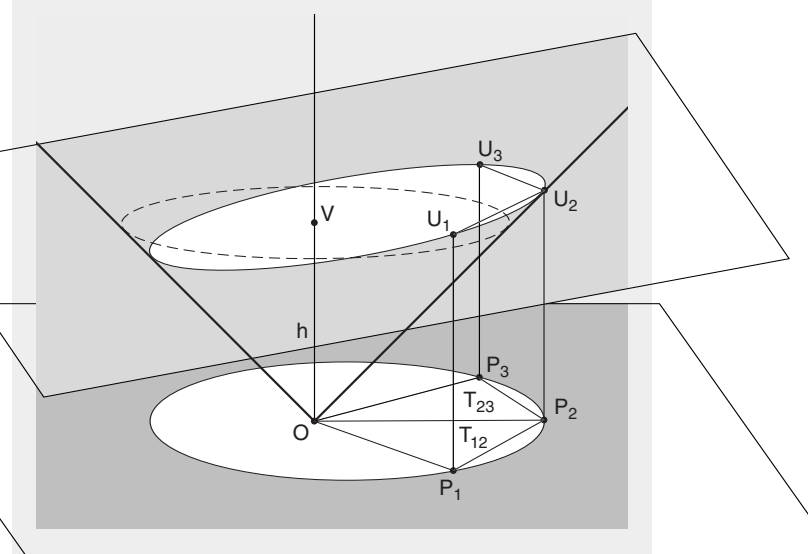
FIGURE 13.3. Our conical projection, which contains both the triangular areas and the elliptical sectors as well as the orbital parameter h , will help us to devise a “fine-tuned” approximation to the crucial coefficients required to determine the orbit of Ceres (cf. Figure 13.1).
