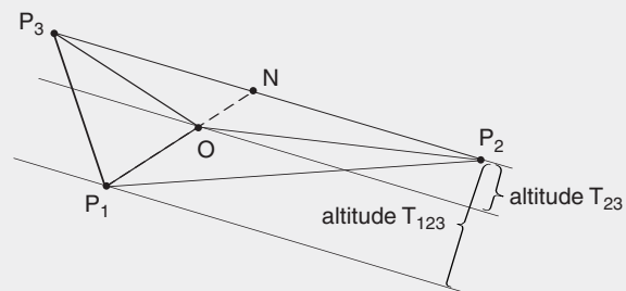
FIGURE 13.7. The division of segment NP_1 by point O is proportional to the ratio of the areas of triangles T_{23} and T_{123} .
